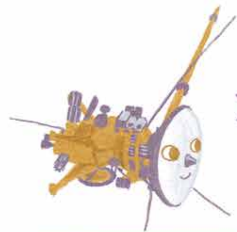
Cassini-Huygens (1997-2017)
